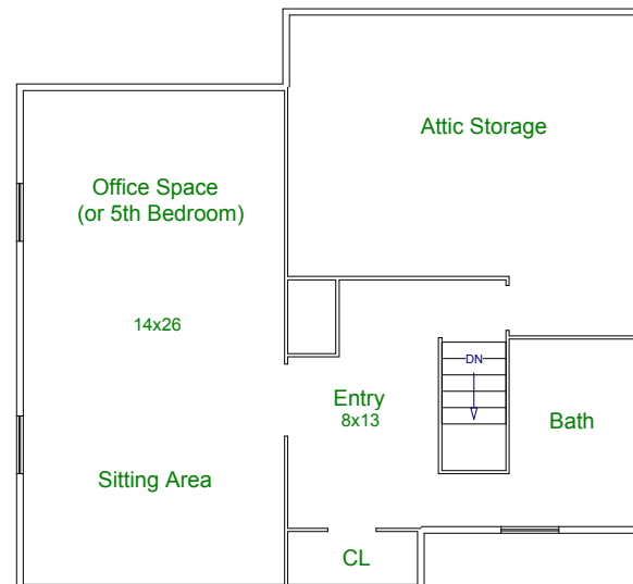
Third Floor
